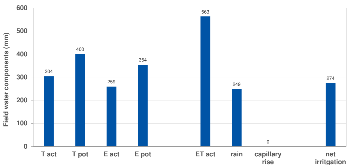
Figure 4.17: FAO-AquaCrop simulated field water components of a practiced drip irrigation (cotton season 2018) at a farm in Samundri region. Raw cotton yield observed was 2.82 ton/ha, simulated 2.75 ton/ha. (Controlled) deficit irrigation utilizing soil storage depletion approaches a realistic upper limit of productivity.
