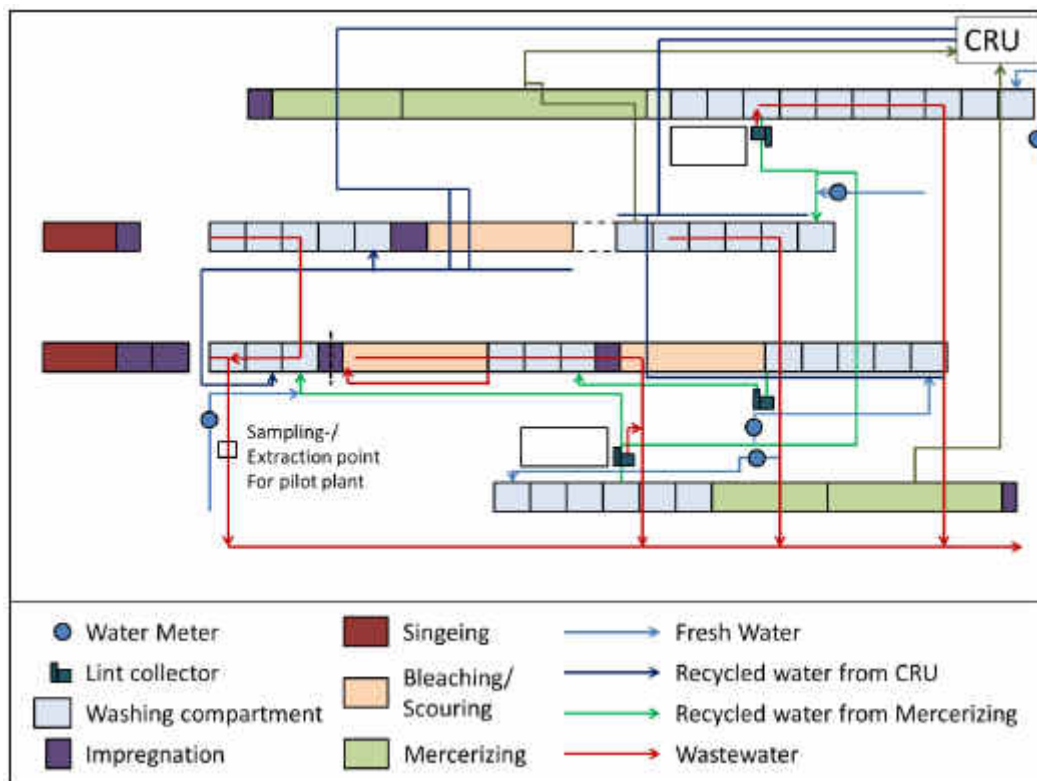
Figure 4.34: Floor plan with fresh water, re-used water and wastewater sewers. © FiW
