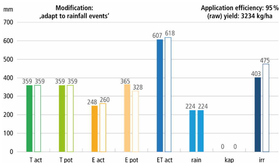
Figure 6.3: AquaCrop modelled field-water balance components of a simulated flexible irrigation schedule integrating / utilizing rainfall to enhance application efficiency (example: drip irrigation).
