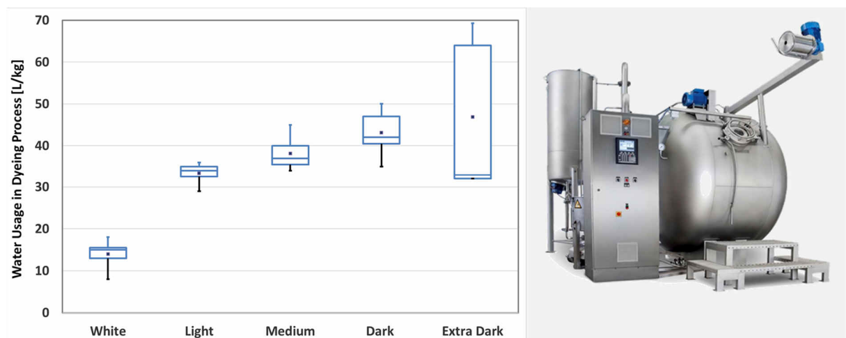
Figure 4.33: Box plots of measured water use of exhaust dyeing machinery THIES iMaster H 2 O operated routinely by textile mills in Pakistan (data base n = 7-9). © THIES
