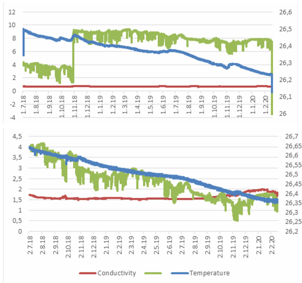
Figure 6.13: Graph with some key results of SEBA LogCom-2 at UAF test site (top) and multi-parameter-sensor MPS-K16 (bottom). © SEBA
