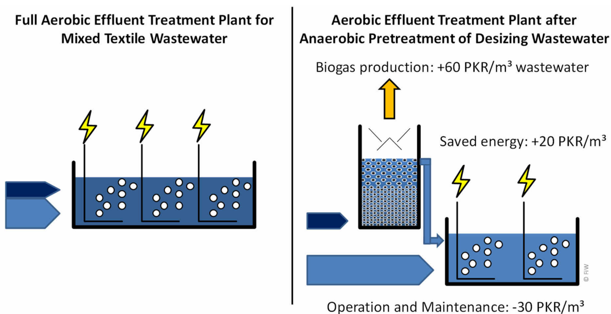
Figure 6.11: Comparison between current aerobic ETP and improved concept with anaerobic pretreatment of desizing wastewater followed by aerobic ETP. © FIW
