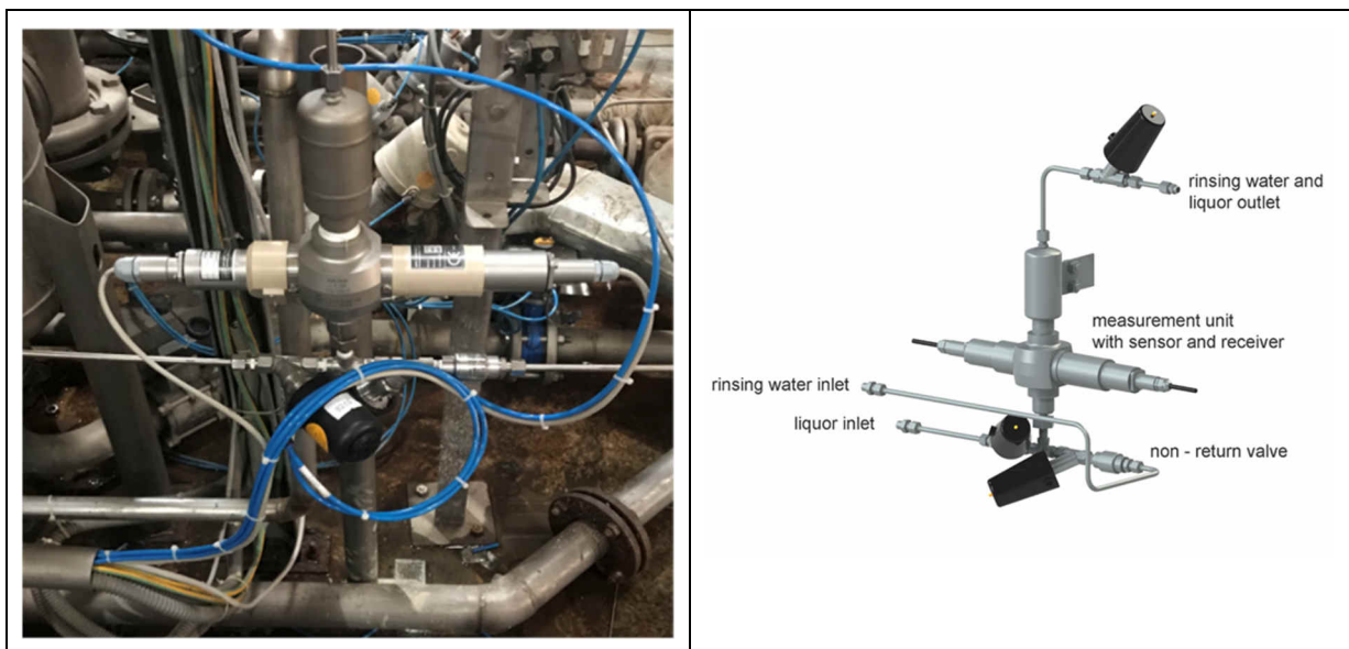
Figure 6.4: Thies DyeControl installed in an existing iMaster H2O exhaust dyeing machinery at a textile finishing plant in Lahore. © Thies
