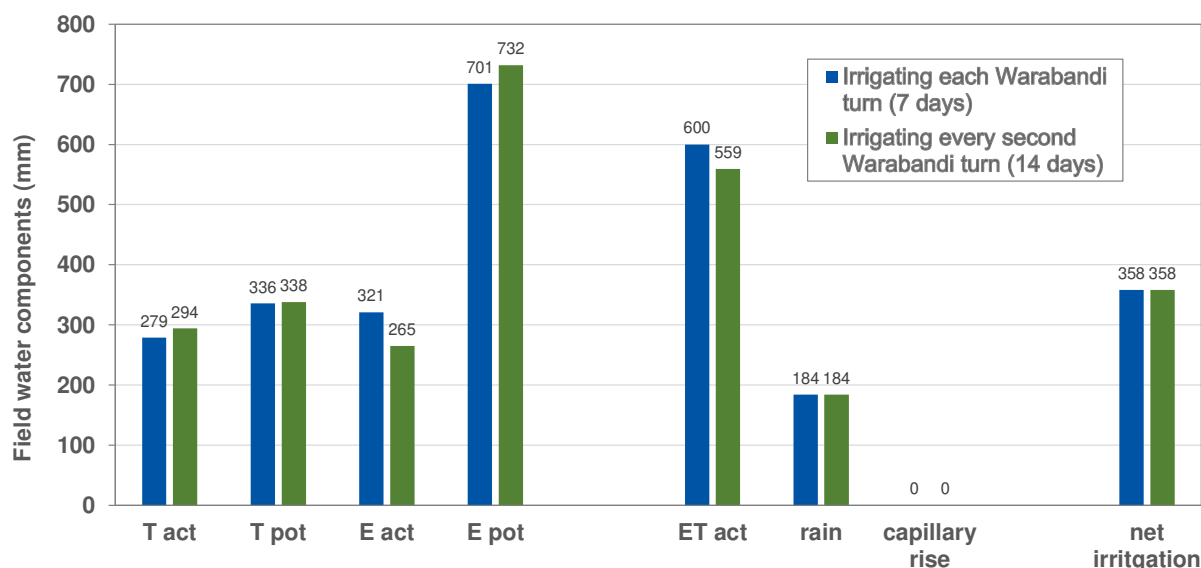
Figure 4.15: Field water components comparing 7-day Warabandi (each turn) to 7-day Warabandi (irrigating only every second turn, 14 days) shifting from (non-productive) evaporation E_{act} to (beneficial) transpiration T_{act} raising raw cotton yield from 2.17 to 2.29 tons per ha.
