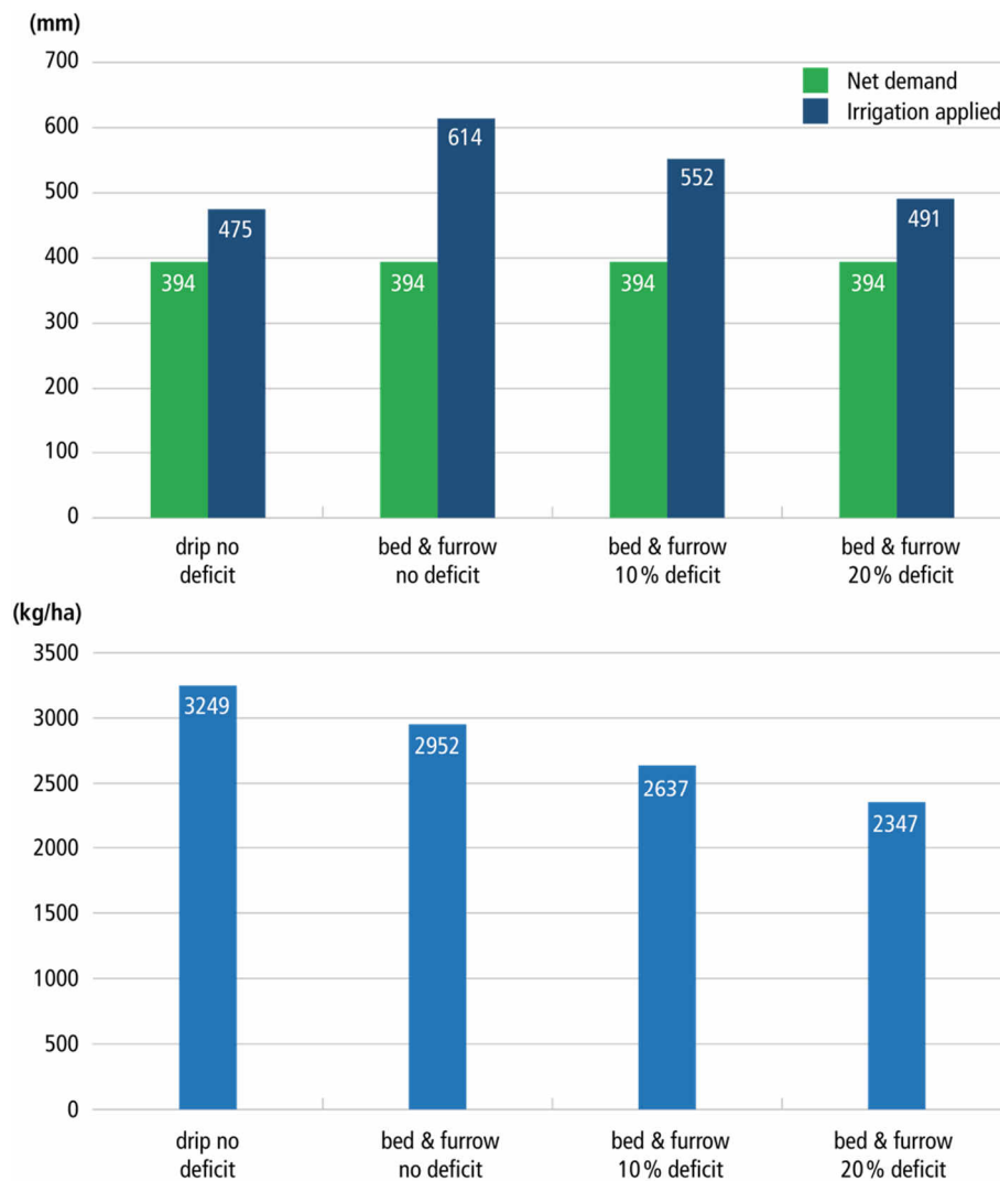
Figure 6.1: Net irrigation demand, gross irrigation applied and recorded yield in irrigation experiments conducted 2017 by UAF at WMRC.
