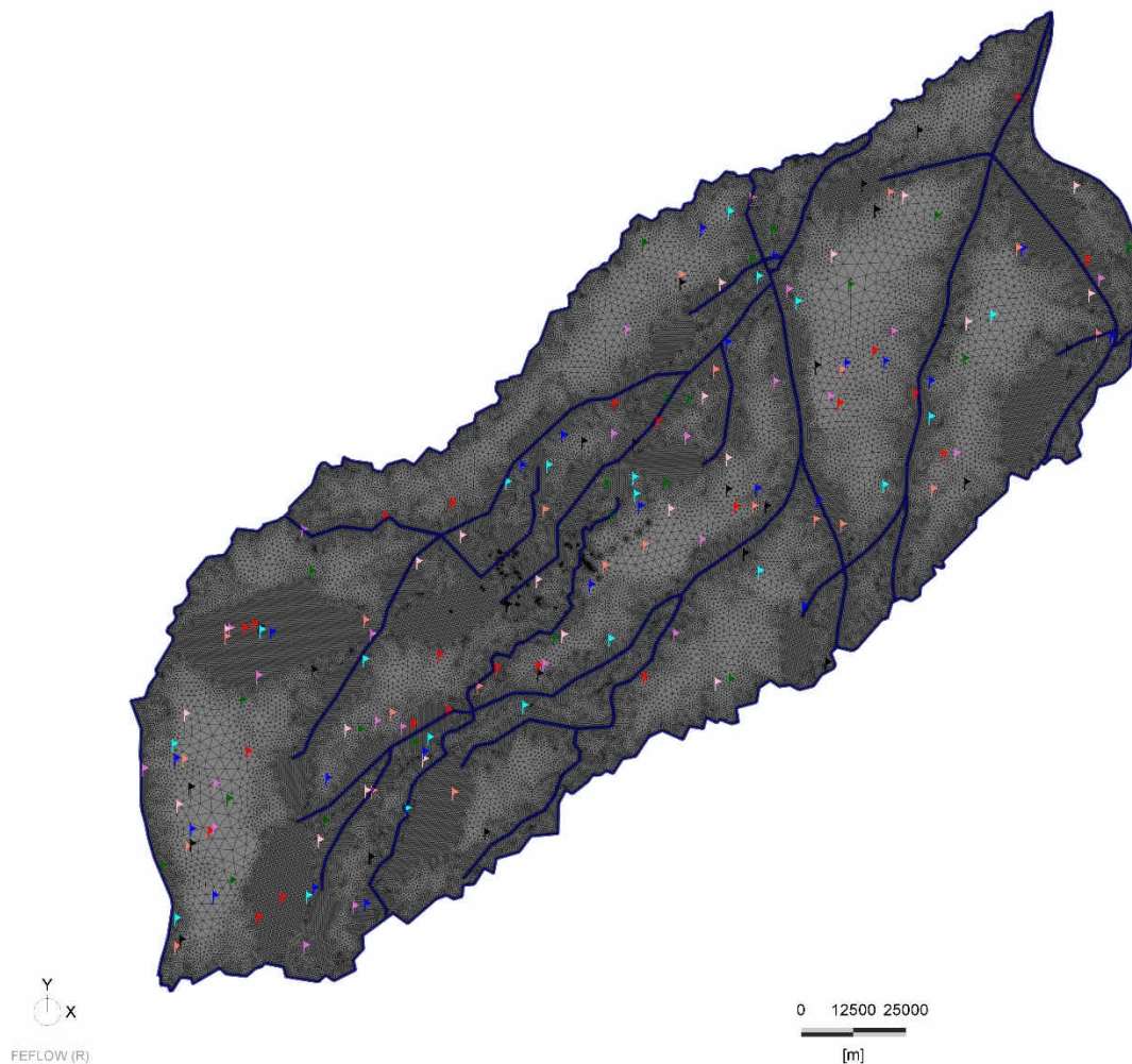
Figure 4.29: Overview of the model area with the triangular finite elements mesh of more than 250.000 nodes. The colored flags represent the locations of the calibration wells. © RWTW-IWW
