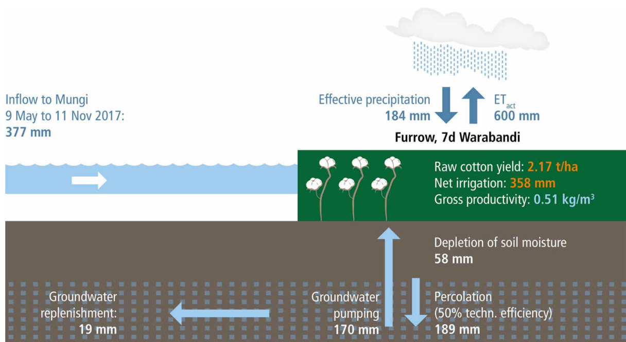
Figure 4.14: Schematic field water balance calculated for 7-day Warabandi for Kharif cotton season from May 9 th to Nov. 11 th , 2017. © FiW
