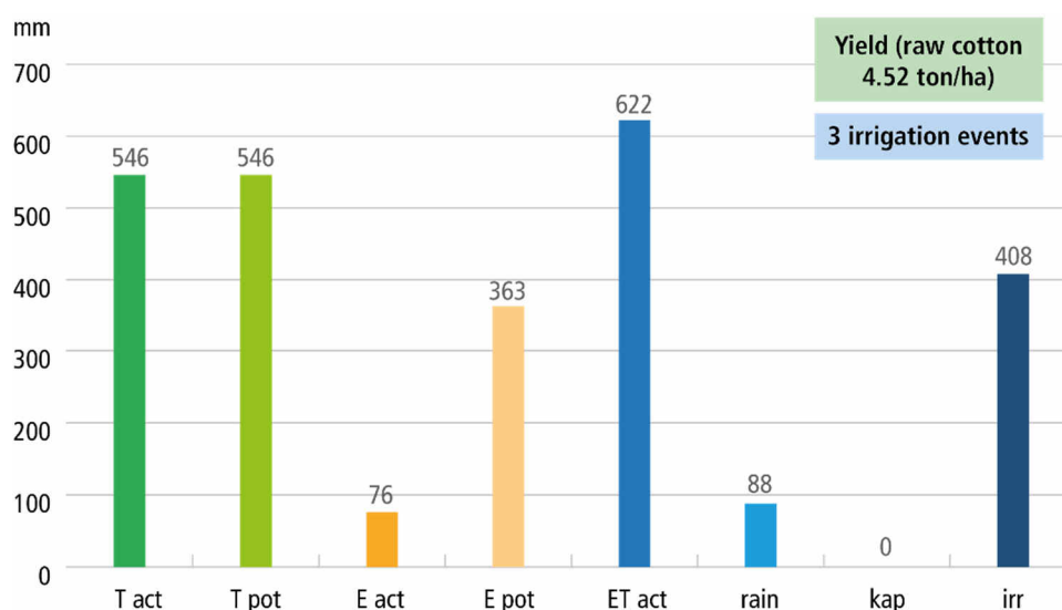
Figure 7.6: Field water balance and irrigation schedule for cotton under the conditions in the WUA Söke (actual and potential transpiration, actual and potential evaporation, evapotranspiration, rain, capillary rise, irrigation).
