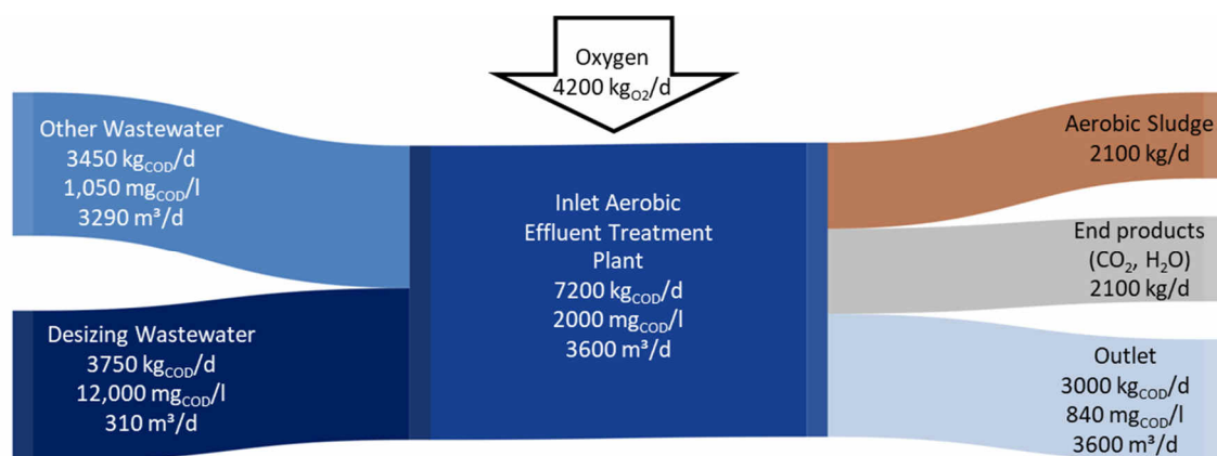
Figure 6.8: Sankey diagram of current COD load streams at the ETP.
